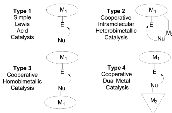
Figure 1. Different approaches to the catalysis of nucleophile (Nu)–electrophile (E) reactions. Geometric shapes (ovals, triangle) symbolize discrete chiral ligands.
